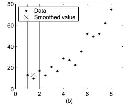
Moving Average Smoothing
